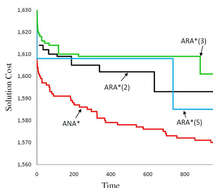
Figure 6: Results for the multiple sequence alignment problem with five protein sequences.
